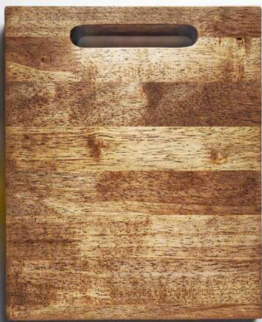
JAVA
